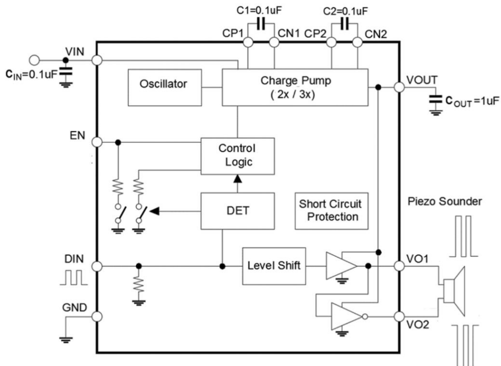
DFN2*2_10 Application
