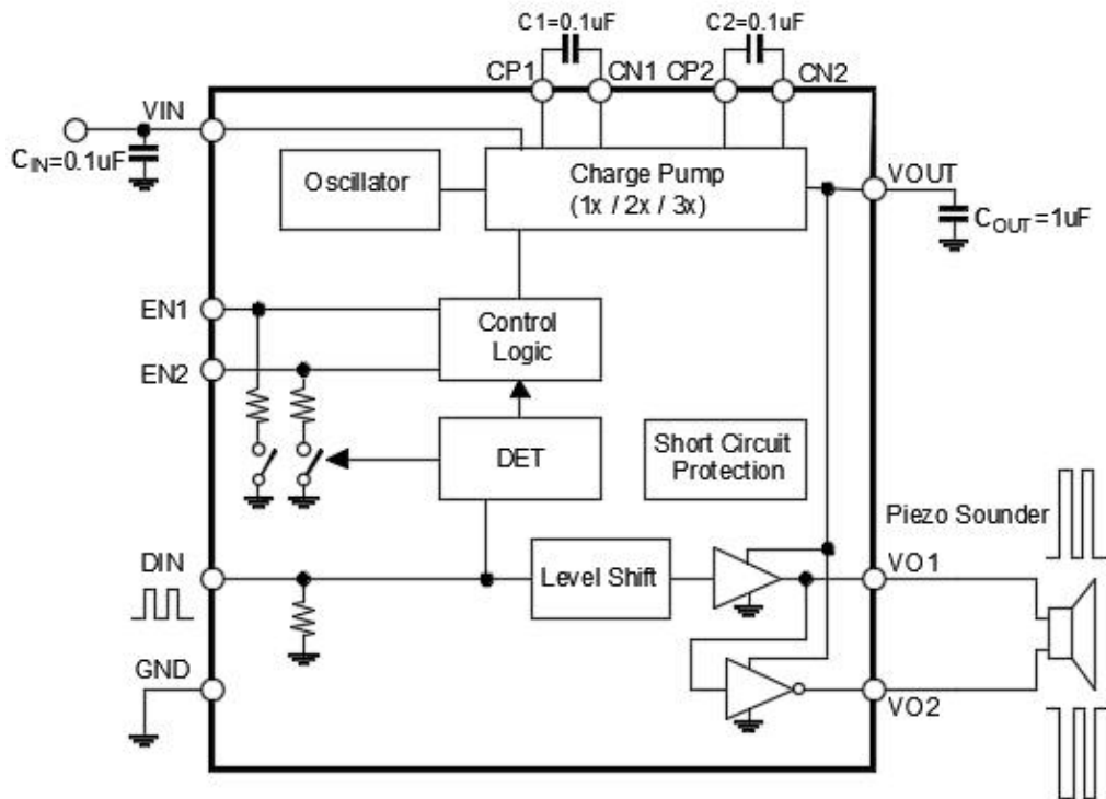
QFN3*3_12/QFN2*2_12/QFN3*3_16 Application
